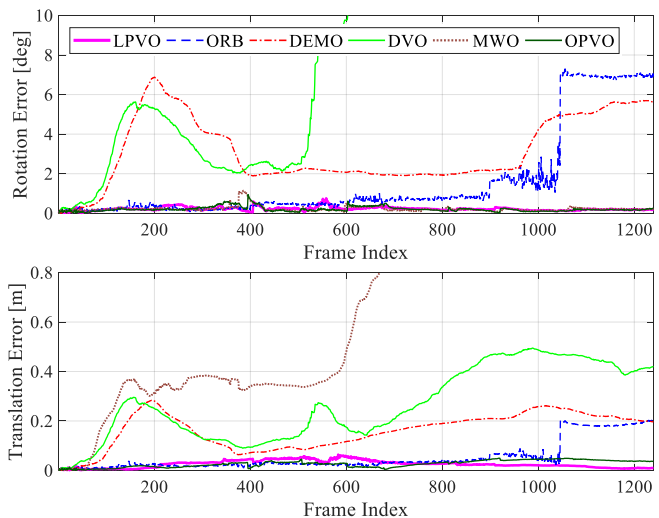
Fig. 6. Absolute rotational error (top) and translational error (bottom) for the proposed and other VO algorithms are plotted. The proposed method shows the lowest rotation and translation error against other VO methods.
