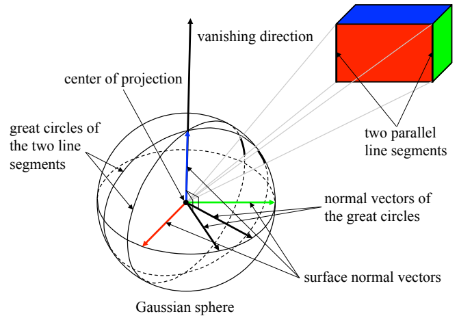
Fig. 2. Background 3D geometric relationship between the lines, planes, and the Gaussian sphere with an orthogonal structure. A vanishing direction vector is defined by at least two parallel line segments. Each orthogonal plane and its corresponding normal vector are drawn with the same color.
