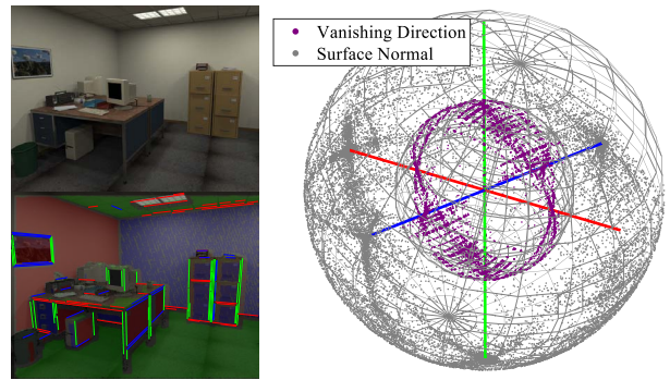
Fig. 3. Clustered lines and segmented planes with inferred MF (left-bottom) are overlaid on the original RGB image (left-top). We employ the concentric spheres (right) with different radius to describe the density distribution of the VDs (purple) and SNs (grey) effectively as 3D points. We can observe that the directional vectors on the both inner (the VDs from lines) and outer (the SNs from planes) sphere are distributed together around the MF axes.
