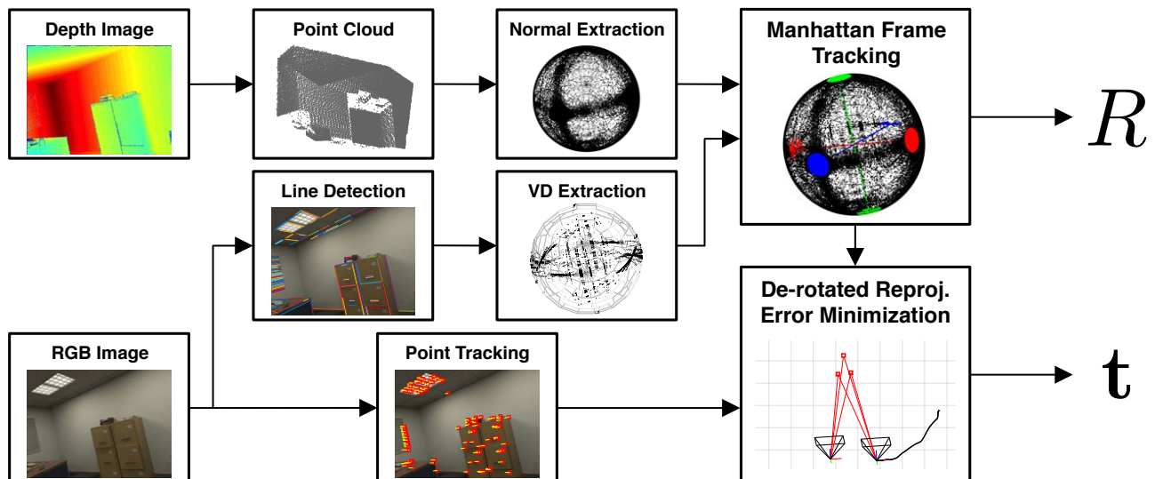
Fig. 4. Overview of LPVO. We estimate the camera rotation ( R ) by tracking the MF from the vanishing directions and surface normals. Once the absolute orientation is known, we recover translational motion ( \mathbf{t} ) by minimizing a de-rotated reprojection error based on tracked points with and without depth.
