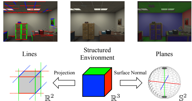
Fig. 1. Example of a structured environment exhibiting strong orthogonal spatial regularities. For drift-free and stable rotation estimation, we exploit line and plane primitives together to recognize the structural regularities with respect to an RGB-D camera.
