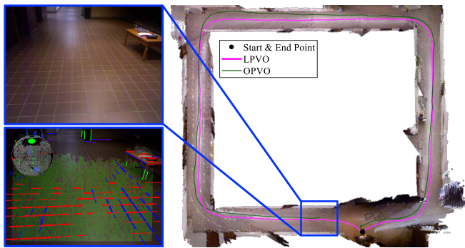
Fig. 8. Example image from ‘Corridor-A-const’, the clustered lines/planes, and the inferred MF orientation are shown on the left. Since an RGB-D camera looks at only a single plane from this blue box point, OPVO fails to estimate camera motion while LPVO does not. The 3D point cloud is rendered by back-projecting the depth sensor from the estimated camera trajectory with the proposed method. No fusion is performed.
