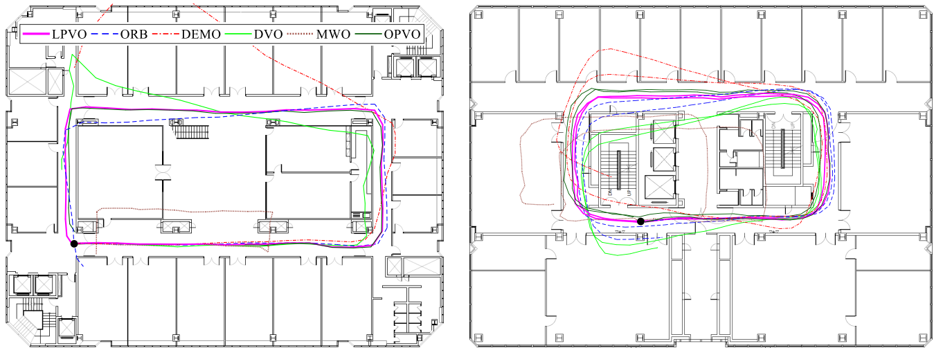
Fig. 10. Estimated trajectories with the proposed and other VO methods on the author-collected dataset in a single-loop (left) and multiple-loop (right) sequences. We start and end at the same point marked in the black circle to check loop closing in the estimated trajectories.
