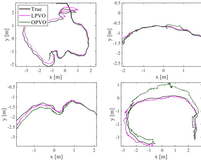
Fig. 7. Estimated trajectories with LPVO (magenta), OPVO (dark green), and ground-truth (black) in the TUM fr3_longoffice, fr3_struc_notex_far, fr3_struc_tex_near, and fr3_large_cabinet.
