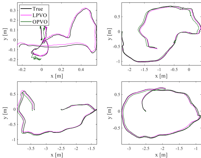
Fig. 5. Estimated trajectories with LPVO (magenta), OPVO (dark green), and ground-truth (black) in the ICL-NUIM dataset Living Room 0, 2 and Office Room 1, 3.
